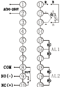
CD900接线图
